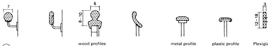
② Handrail profiles
